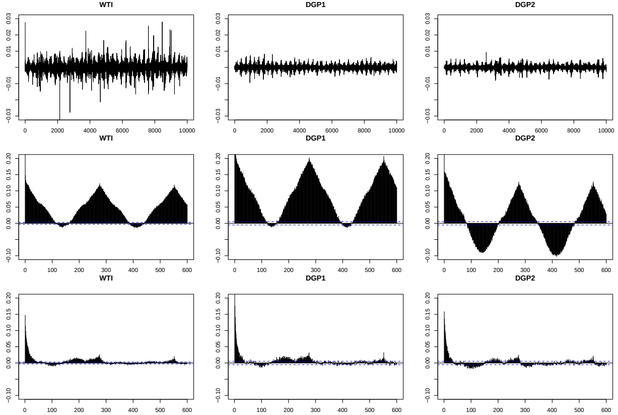
Figure 9: Real and simulated datasets. First row: first 10k observations of log-returns y_t . Second and third rows: ACFs and PACFs of \log(y_t^2) .
