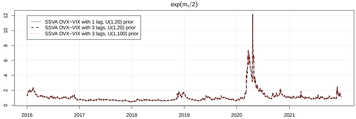
Figure 7: The evolution of MIDAS component in terms of standard deviation \exp(m_\tau/2) for the in-sample period, estimated at the posterior modes of model parameters for the SSVA OVX-VIX model with one lag, three lags and three lags and wide prior for the weights.
