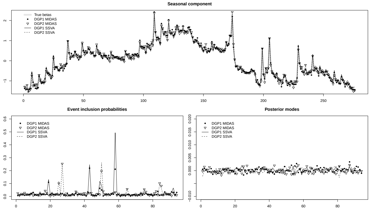
Figure 10: Simulation study results. Top panel: estimated posterior median seasonal component for MIDAS and SSVA models for both simulated DGPs, compared to the true seasonal betas (gray). Bottom-left panel: posterior mean event inclusion probabilities. Bottom-right panel: posterior mode event coefficients. True event values are zero for all DGPs.
