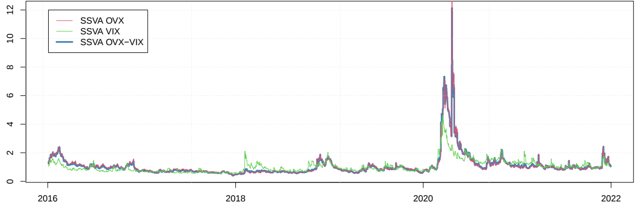
Figure 1: The evolution of MIDAS component in terms of standard deviation \exp(m_\tau/2) for the in-sample period, estimated at the posterior modes of model parameters.
