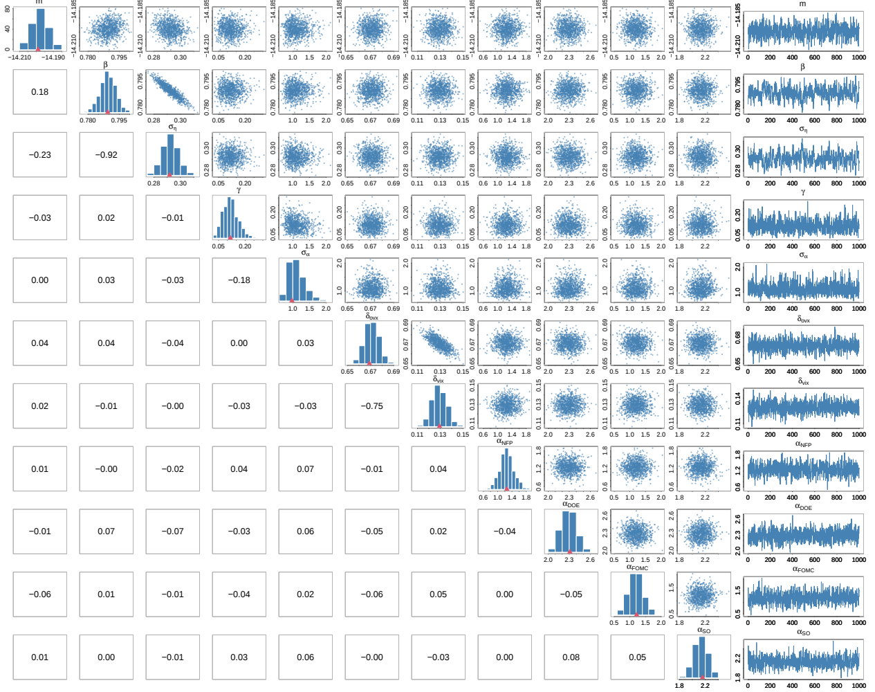
Figure 5: Posterior density plots, trace plots and scatterplots for the parameters in a SSVA MIDAS model with OVX and VIX variables in scaled-log-levels. The red triangles are the posterior modes.
