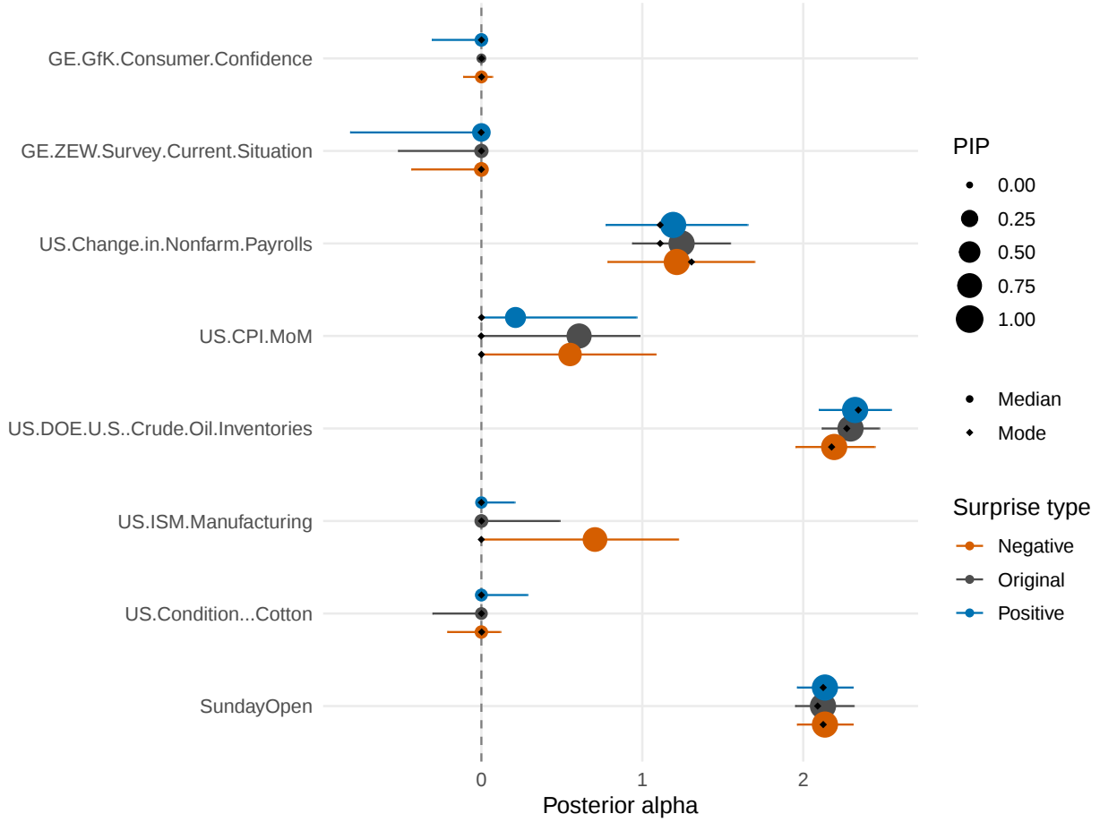
Figure 8: Summary of the estimated posterior parameters associated with the selected events and their posterior inclusion probabilities (PIP). The colored round dots are posterior medians, the small black diamonds are posterior modes and the horizontal colored lines represent the 90% credible intervals.
