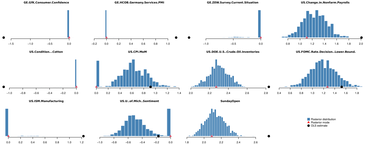
Figure 6: Posterior distributions for the selected events for the SSVA OVX-VIX model. Red triangle is the posterior MCMC mode, black dot is the OLS estimate.
