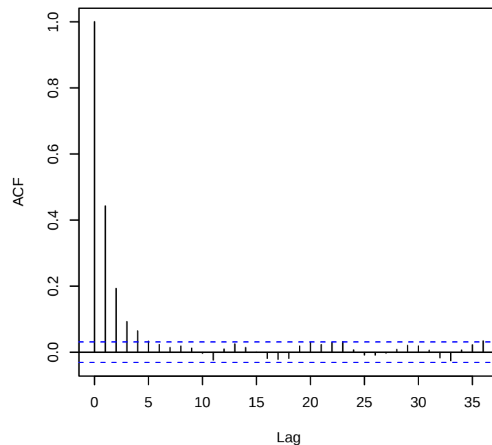
Runtime=0.622sec
