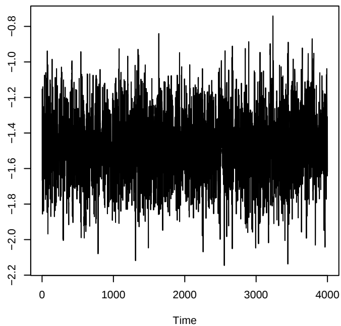
R package stan_glm
