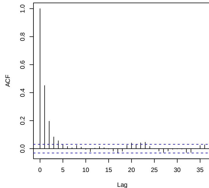
Runtime=3.168sec
