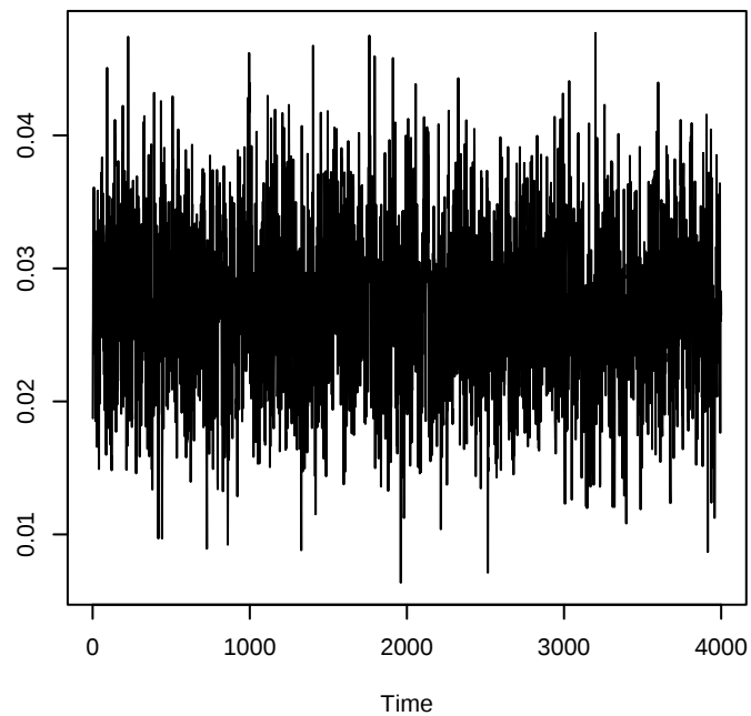
R package UPG
