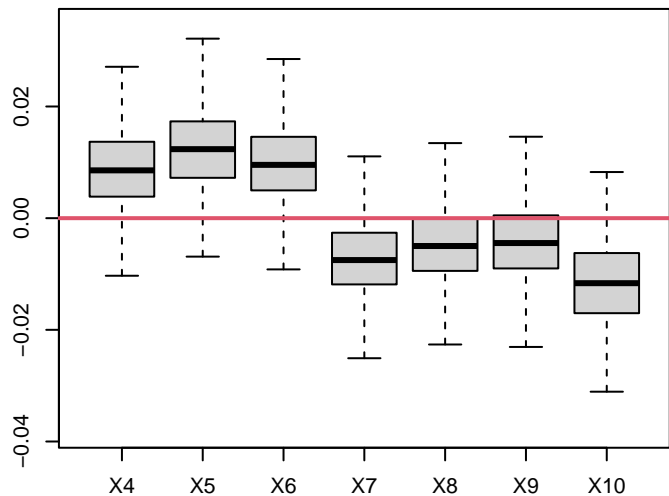
n=200- k=10
