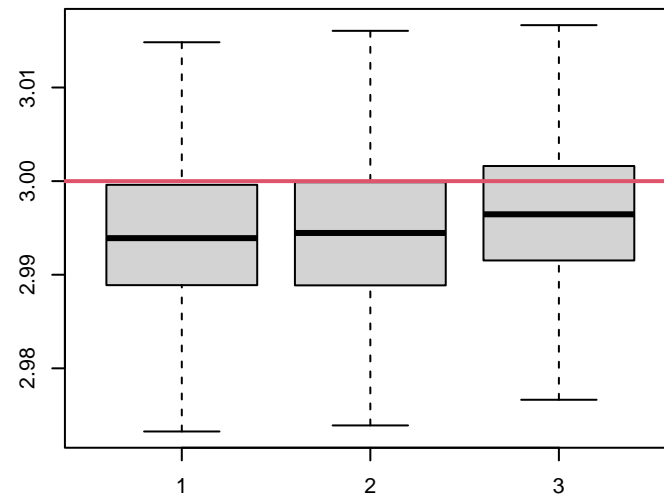
horseshoe
