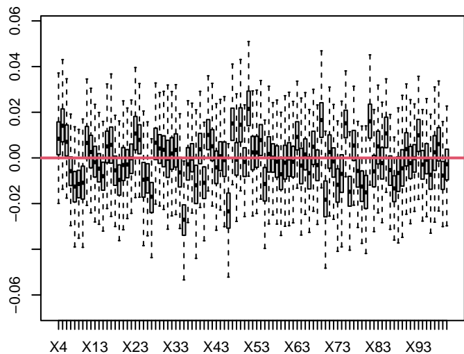
n=200- k=100
