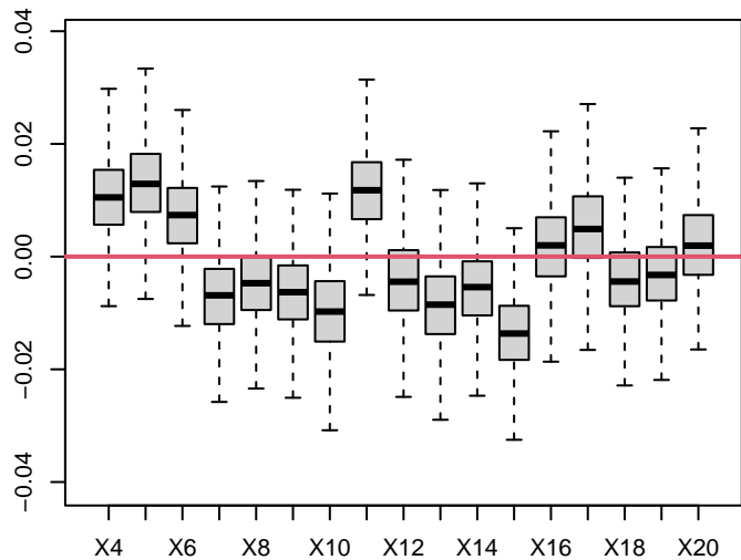
n=200- k=20
