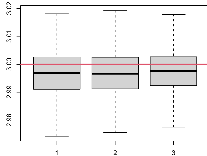
horseshoe
