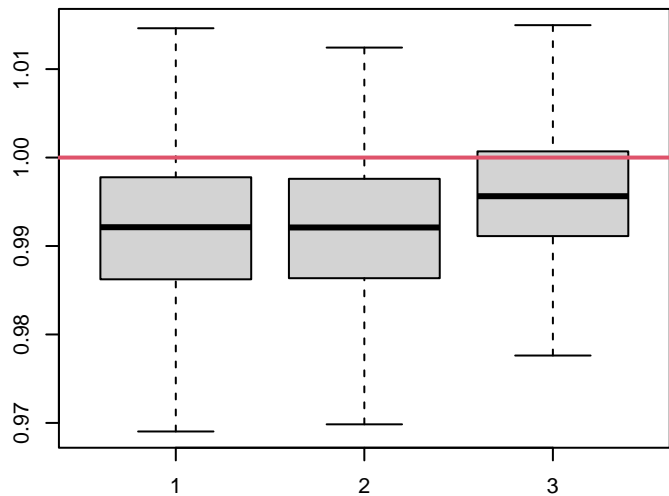
ridge
