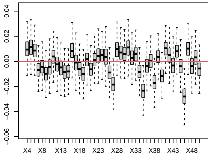
n=200- k=50
