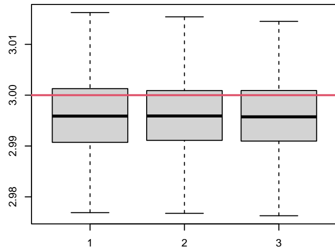
horseshoe
