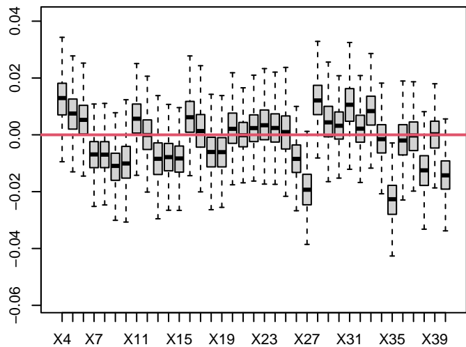
n=200- k=40
