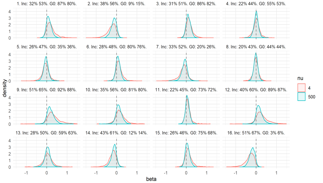
Figure 9: Posterior distribution of beta for the Finance 1 dataset for the t-student prior distribution.
