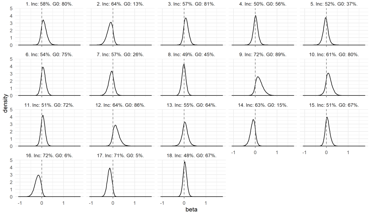
Figure 6: Posterior distribution of beta for the Finance 1 dataset with additional random variables.
