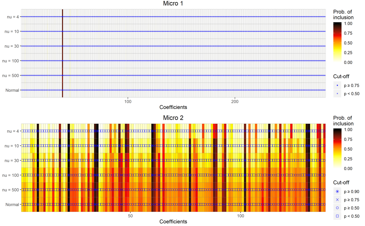
Figure 8: Probability of inclusion of each predictor for the Micro 1 and 2 datasets. Each columns is a predictor and each row one model, varying the number of degrees of freedom \nu .
