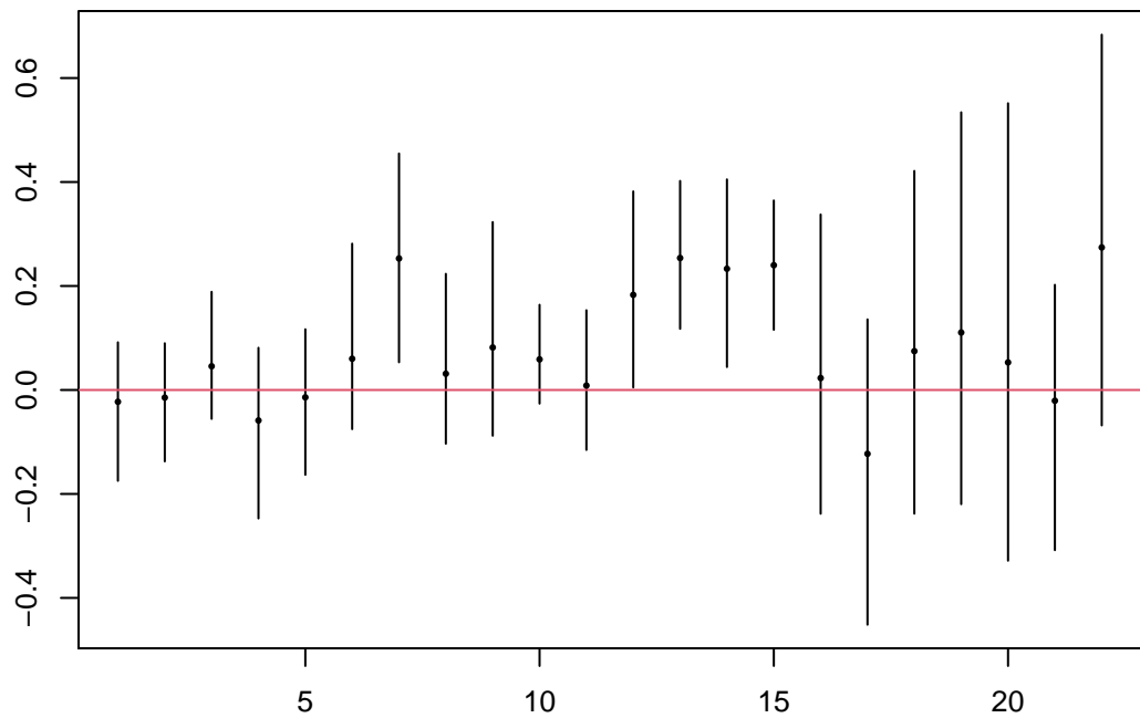
Laplace prior k=5
