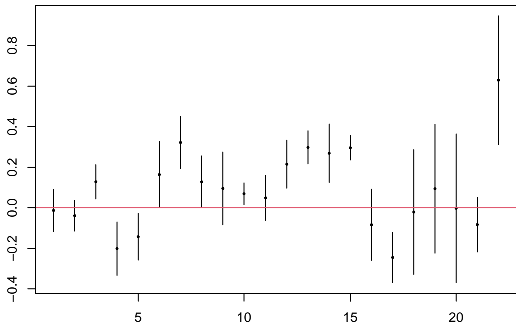
OLS k=13
