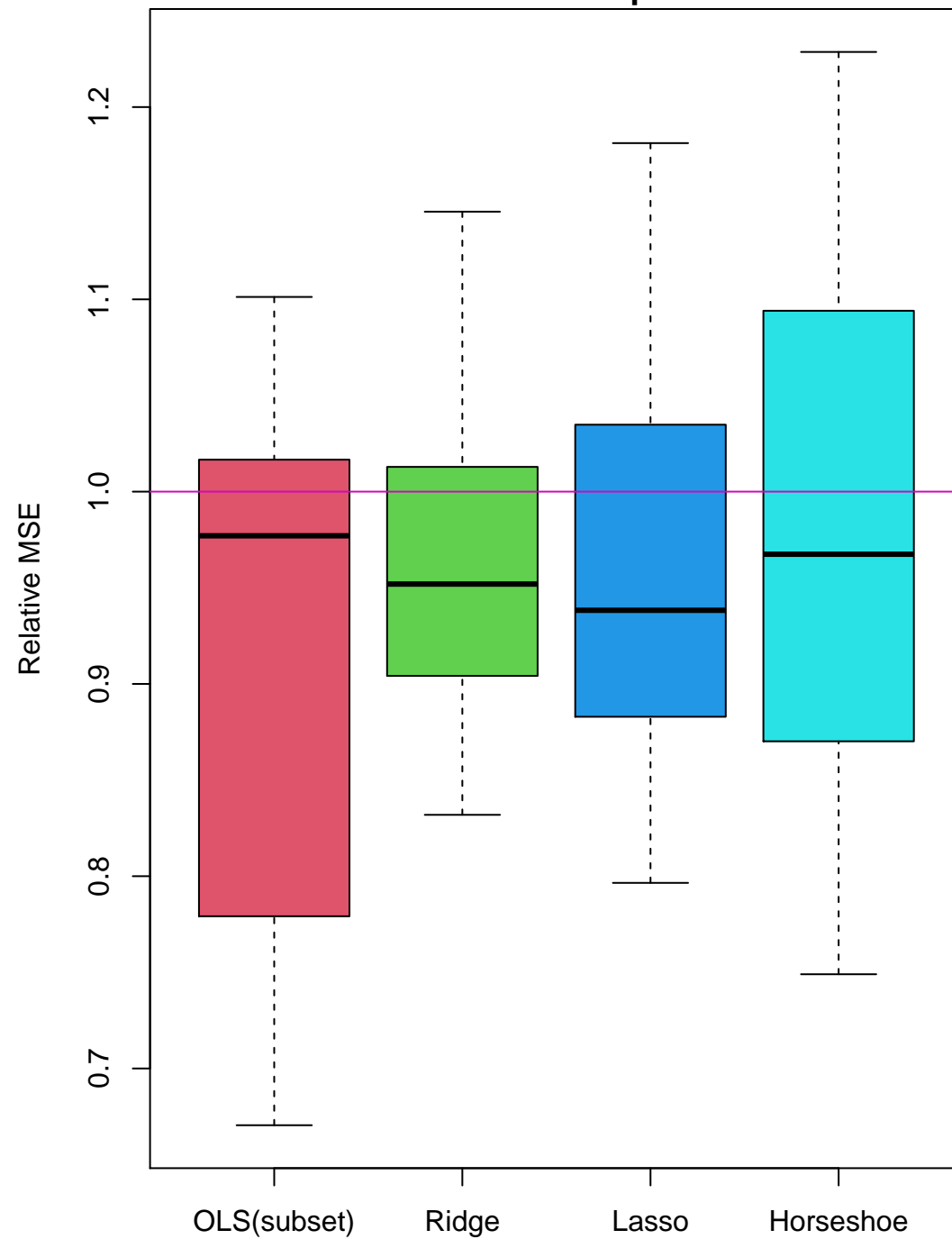
14-fold cross validation Out-of-sample
