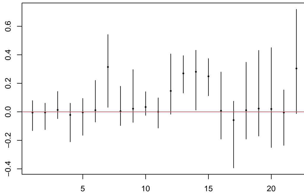
Horseshoe prior k=4
