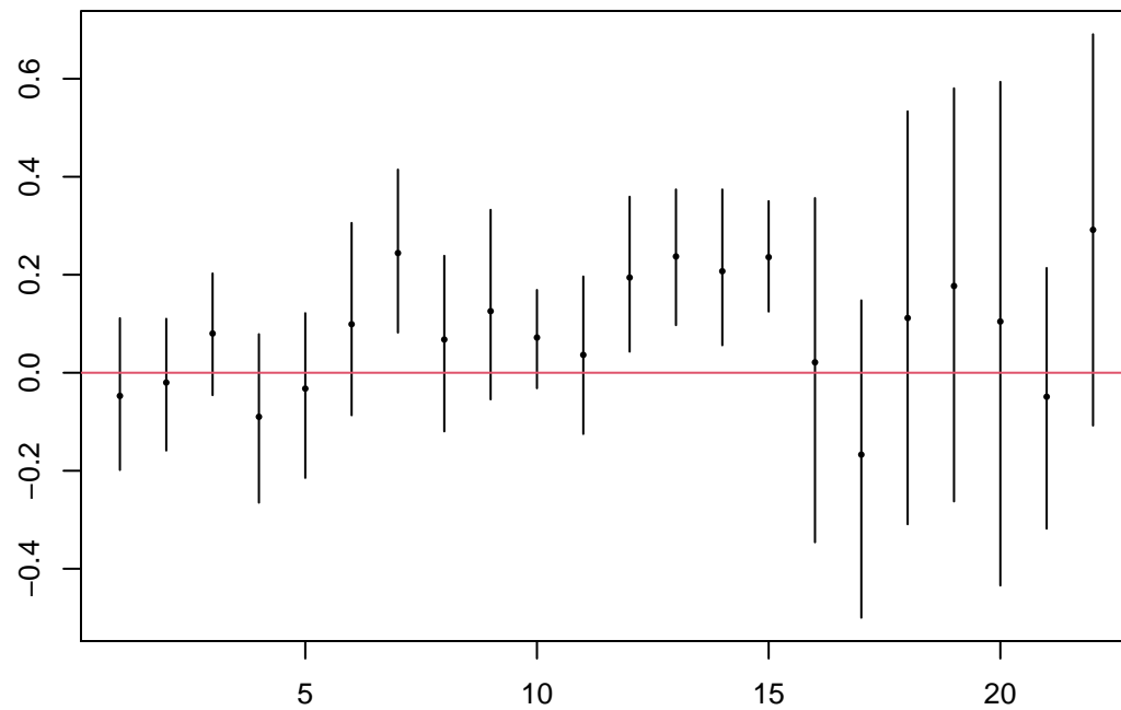
Ridge prior k=5
