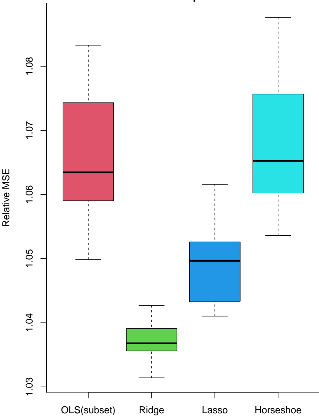
14-fold cross validation In sample
