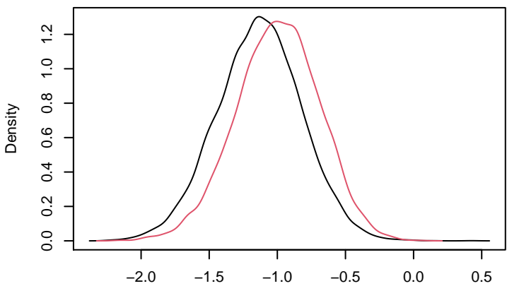
beta(38)
