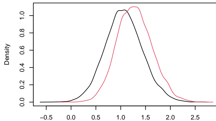
beta(13)
