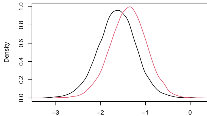
beta(87)
