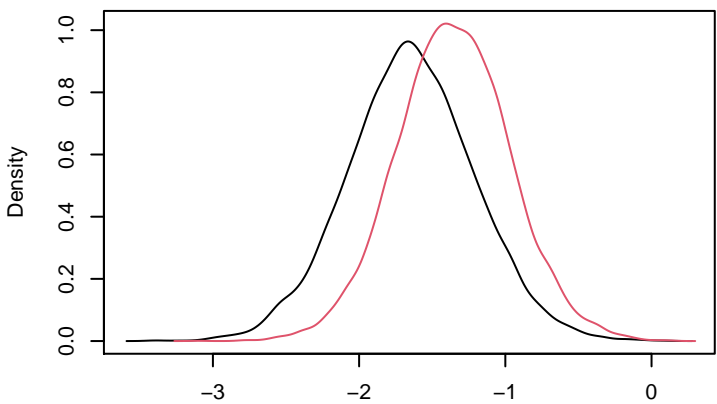
beta(75)
