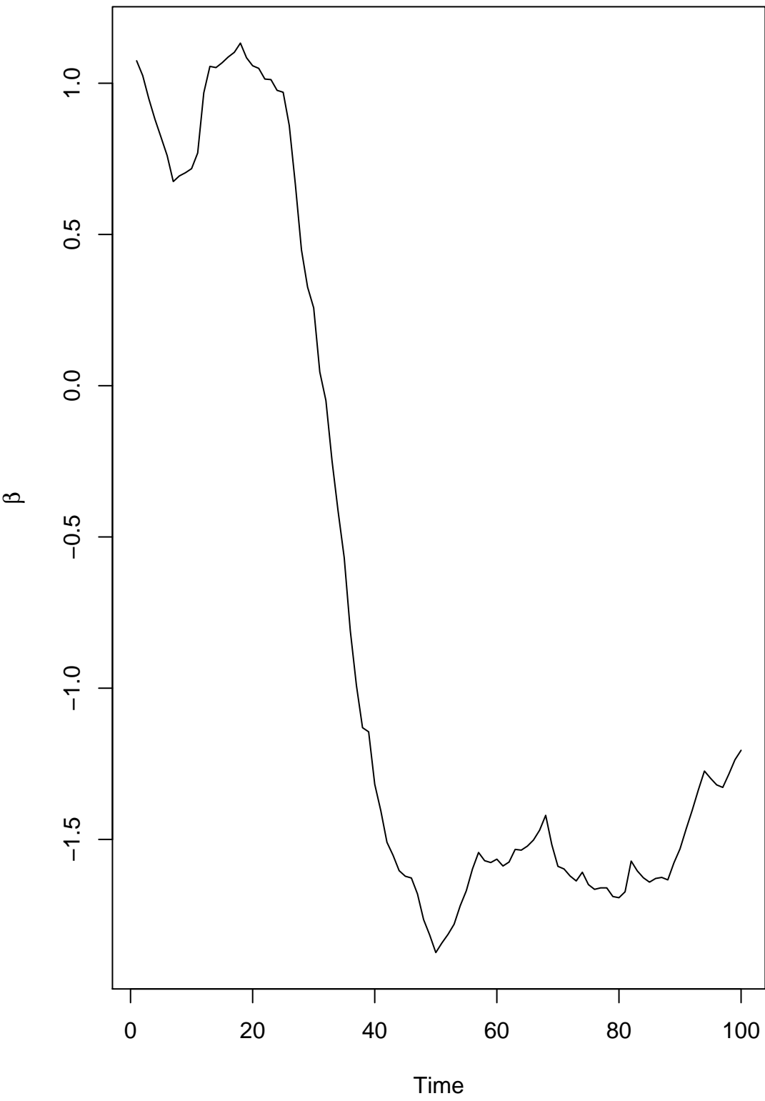
Time-varying coefficient
