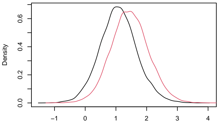
beta(1)
