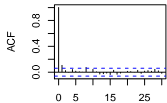
alpha1
