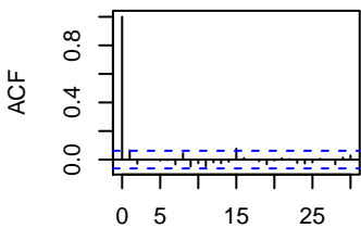
alpha0
