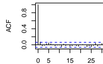
xi
