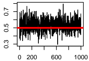
alpha0
