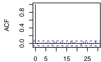
beta
