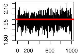
beta
