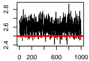
alpha1
