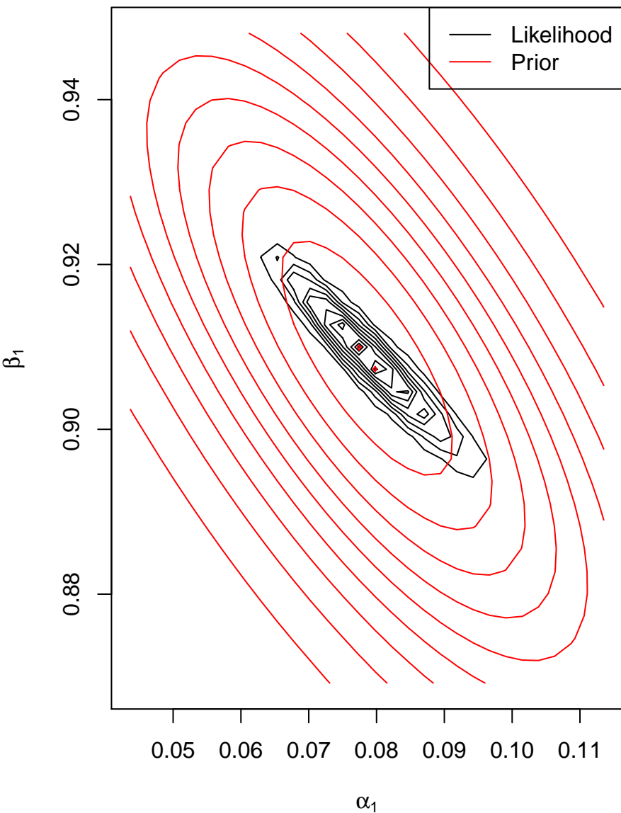
Likelihood & prior contours
