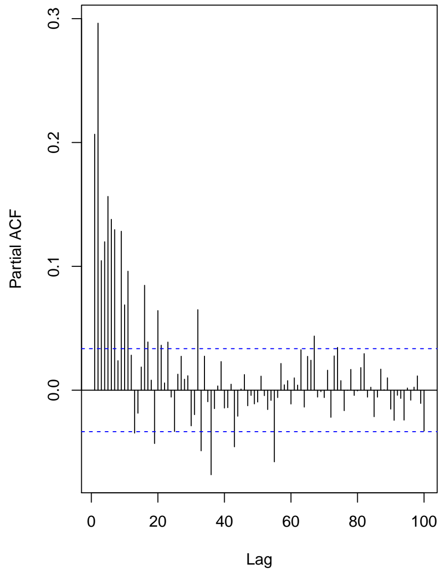
Squared log returns
