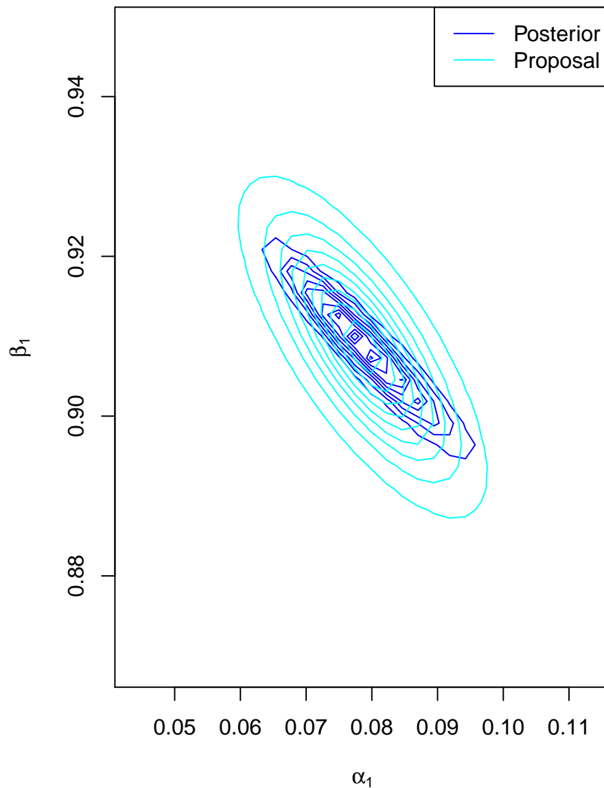
Posterior and proposal contours
