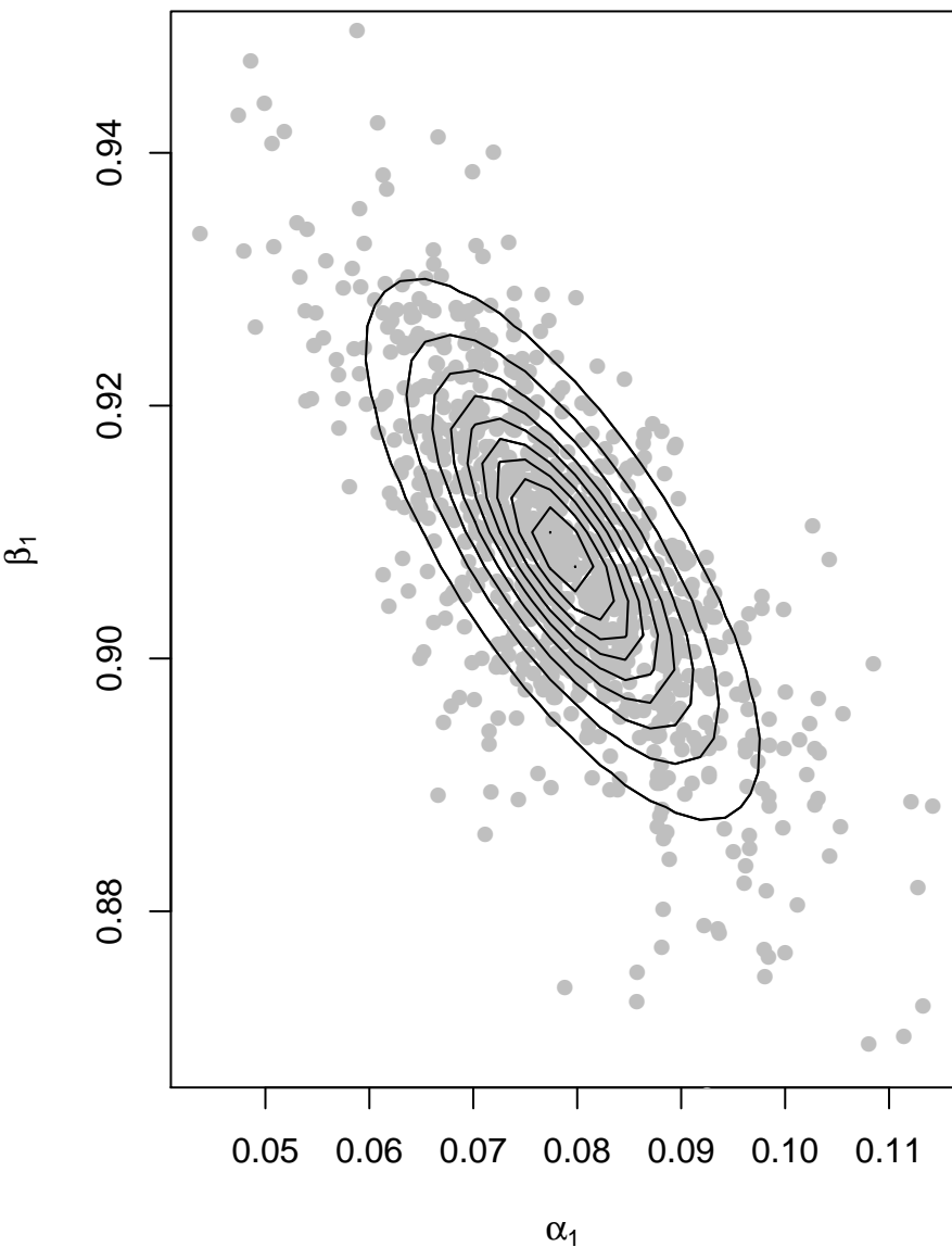
Proposal contours and draws
