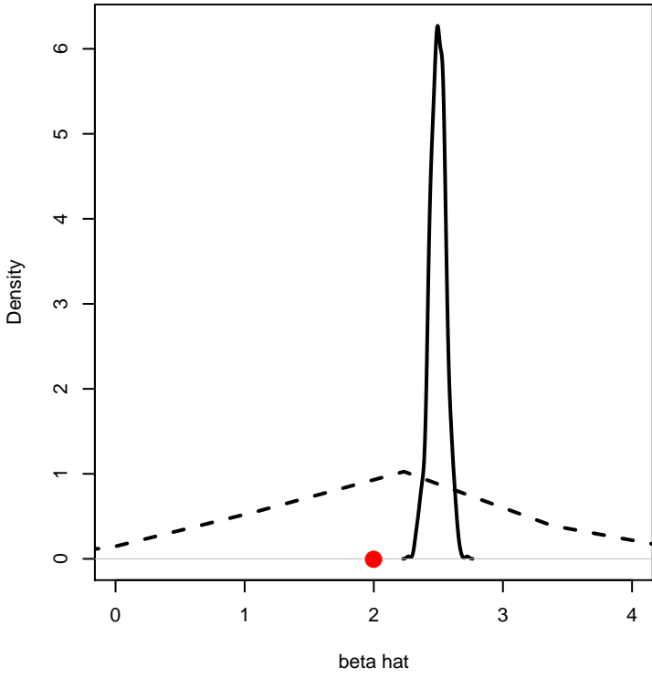
rho=0.5 - delta=0.1 OLS (solid), 2SLS (dashed)
