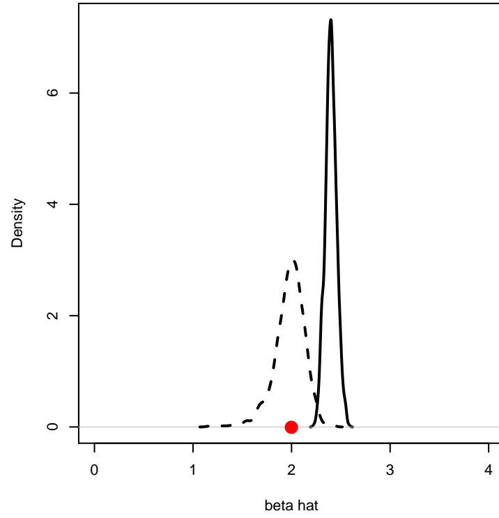
rho=0.5 - delta=0.5 OLS (solid), 2SLS (dashed)
