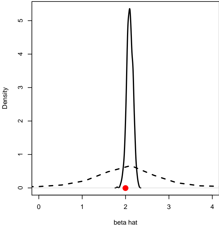
rho=0.1 - delta=0.1 OLS (solid), 2SLS (dashed)
