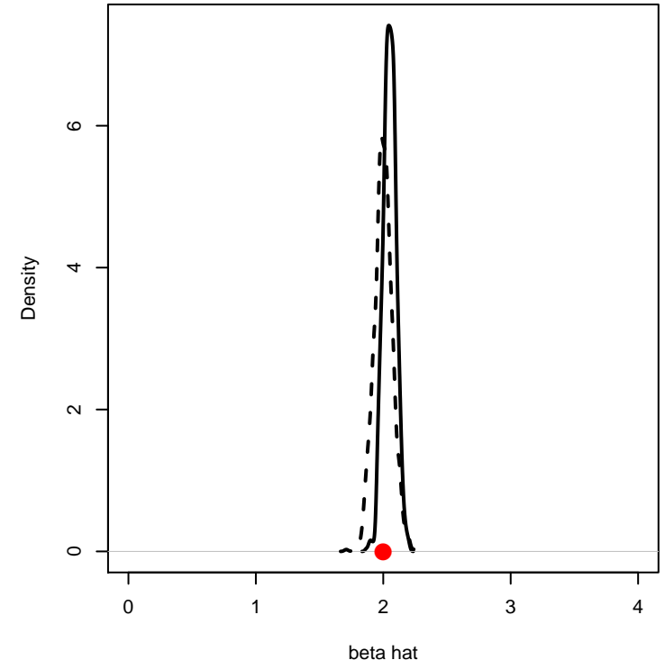
rho=0.1 - delta=1 OLS (solid), 2SLS (dashed)
