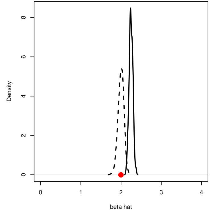
rho=0.5 - delta=1 OLS (solid), 2SLS (dashed)
