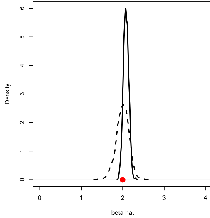
rho=0.1 - delta=0.5 OLS (solid), 2SLS (dashed)
