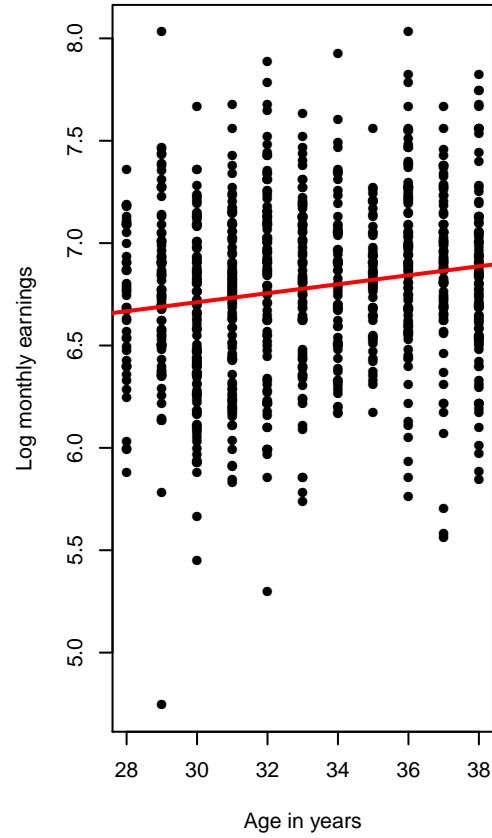
Correlation=0.162
