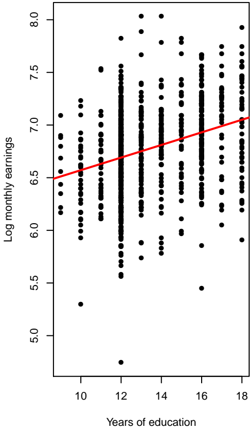
Correlation=0.312
