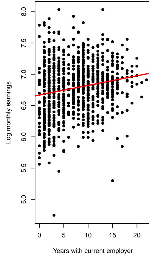
Correlation=0.186
