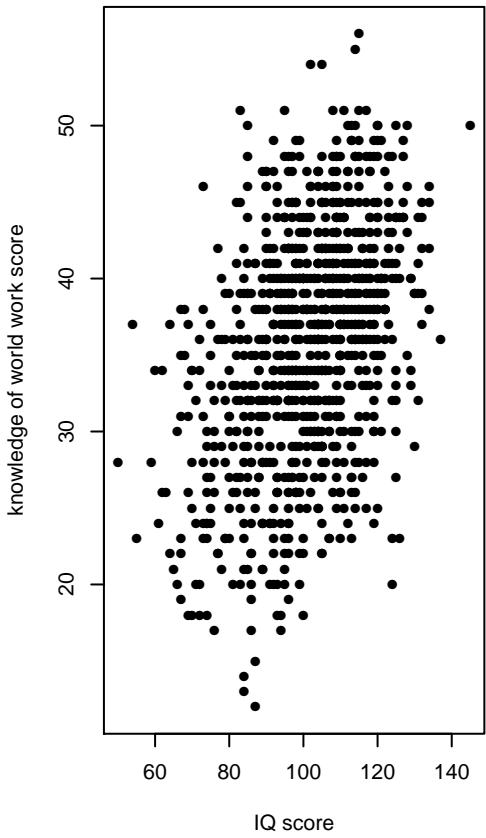
Correlation=0.414
