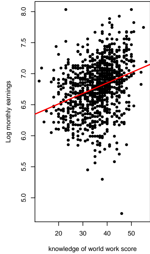
Correlation=0.306
