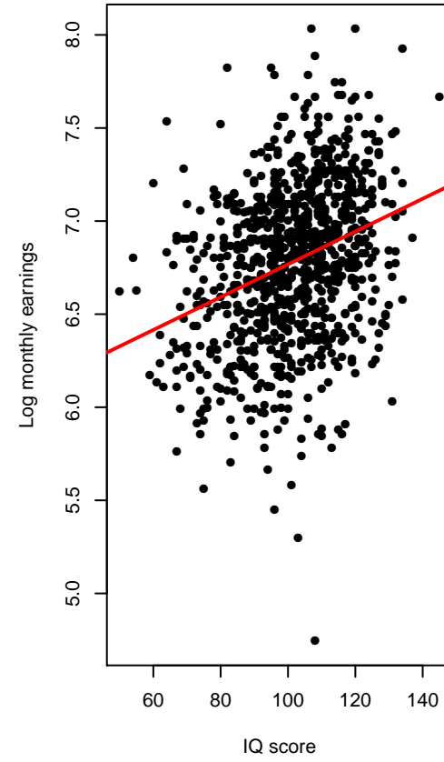
Correlation=0.315
