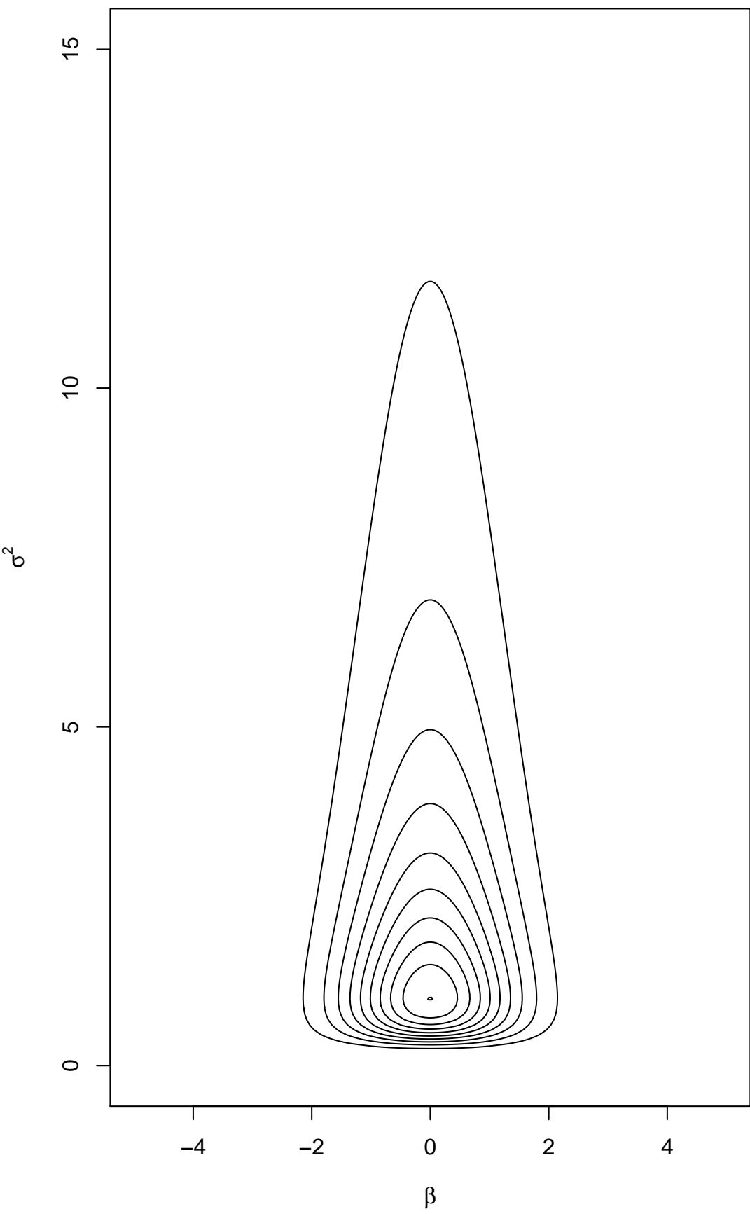
Prior
