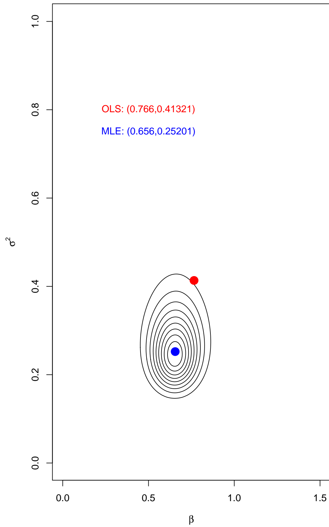
Likelihood
