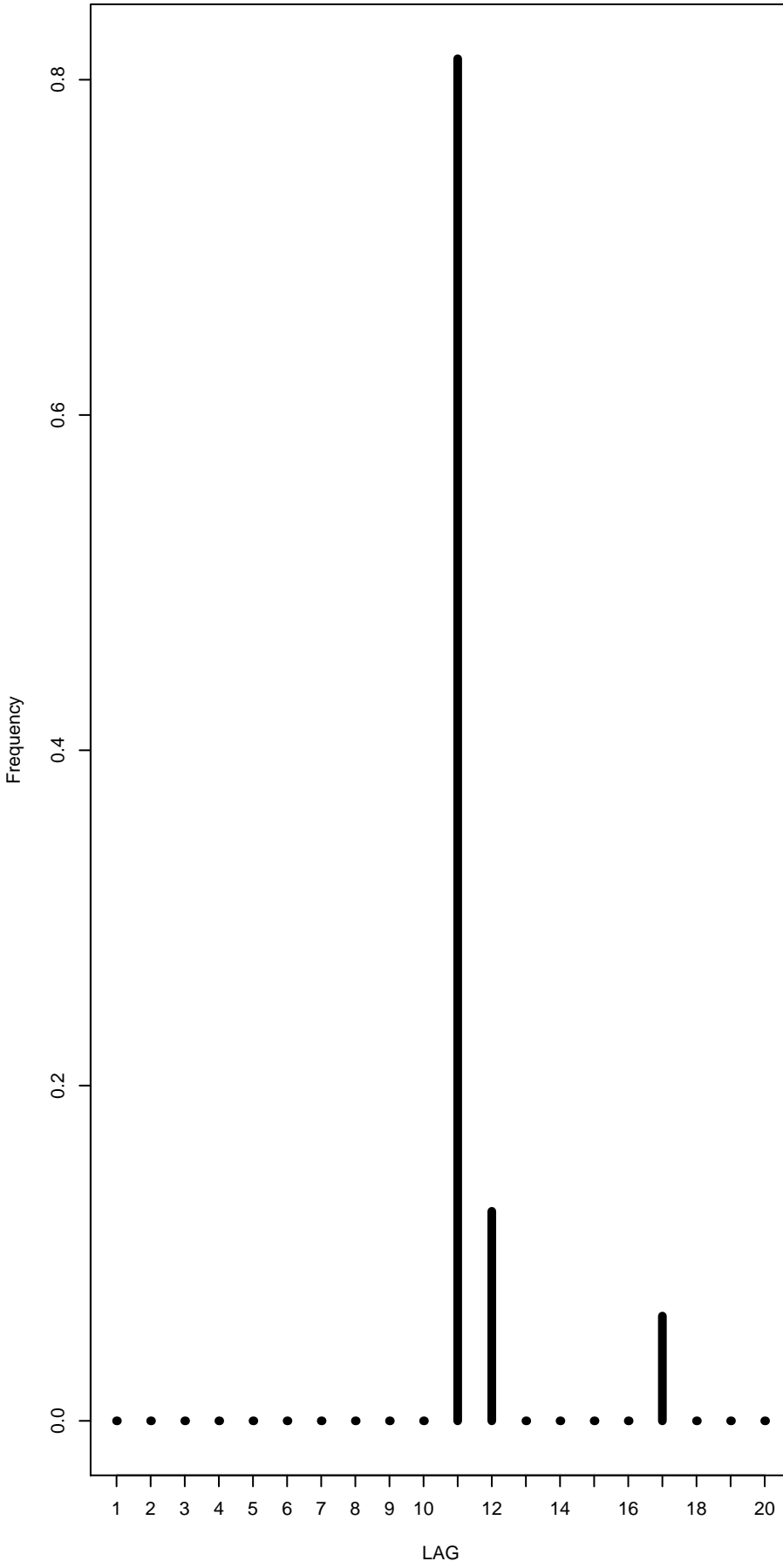
BAYES n=600
