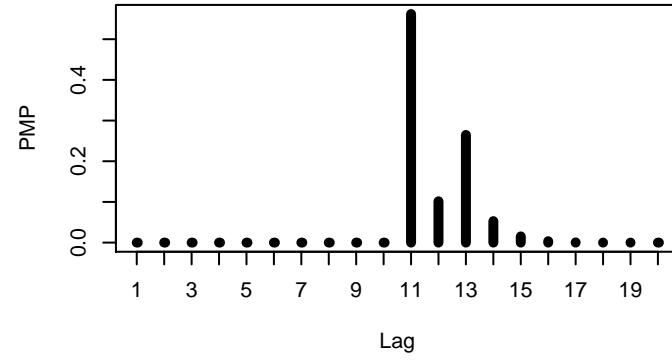
dataset 6 n=600
