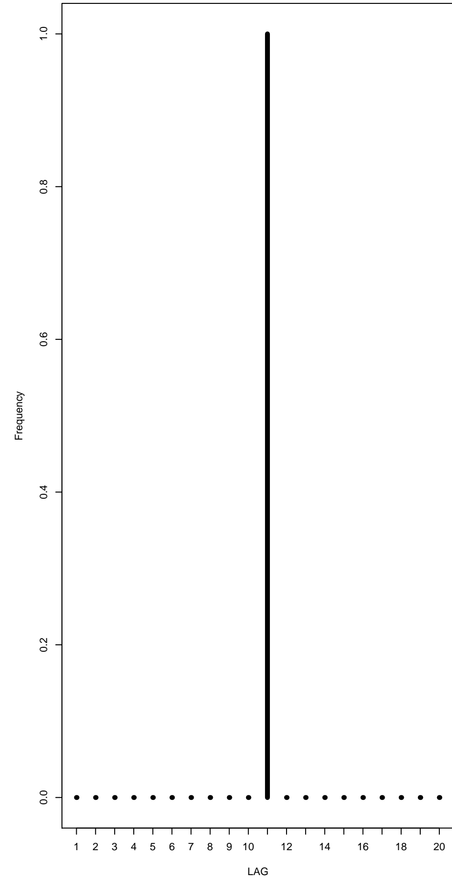
BIC n=1200
