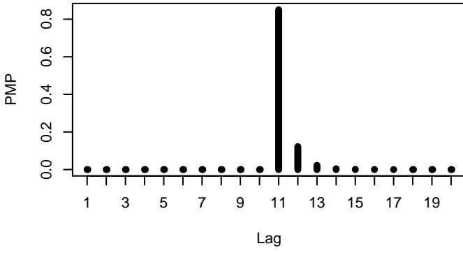
dataset 5 n=600
