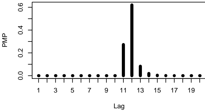
dataset 9 n=600
