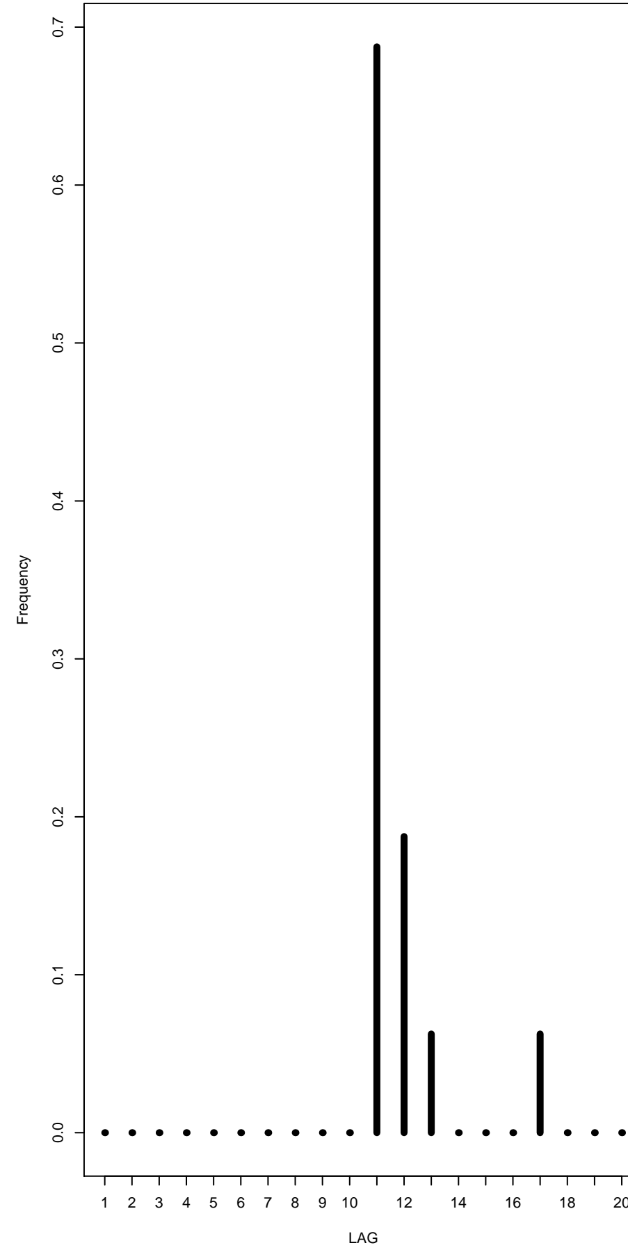
AIC n=600
