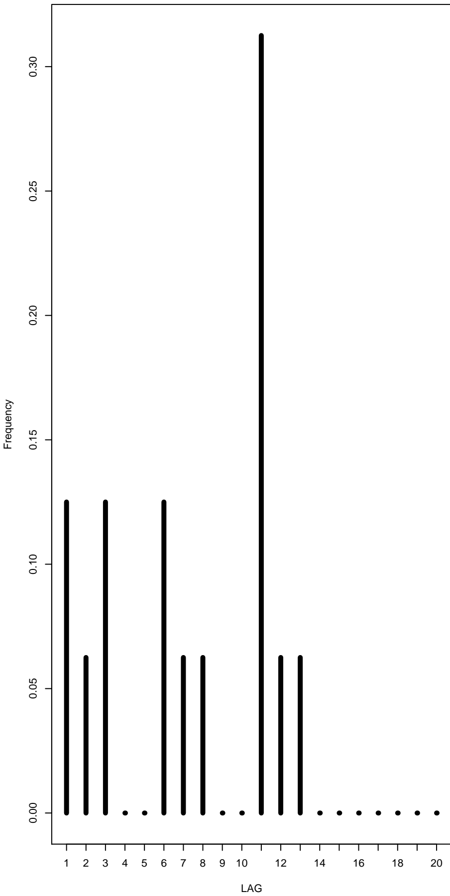
BAYES n=120
