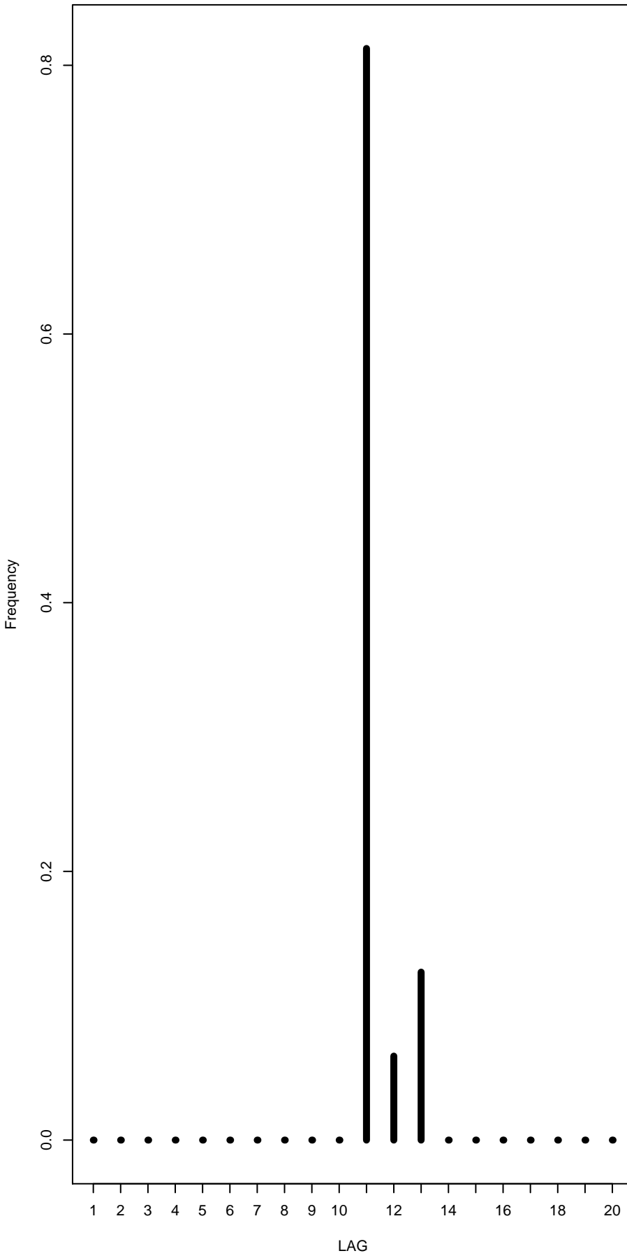
BAYES n=1200
