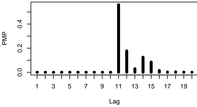
dataset 1 n=600
