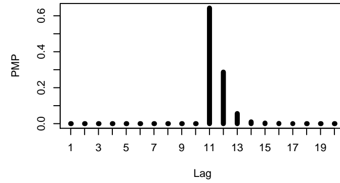
dataset 15 n=600
