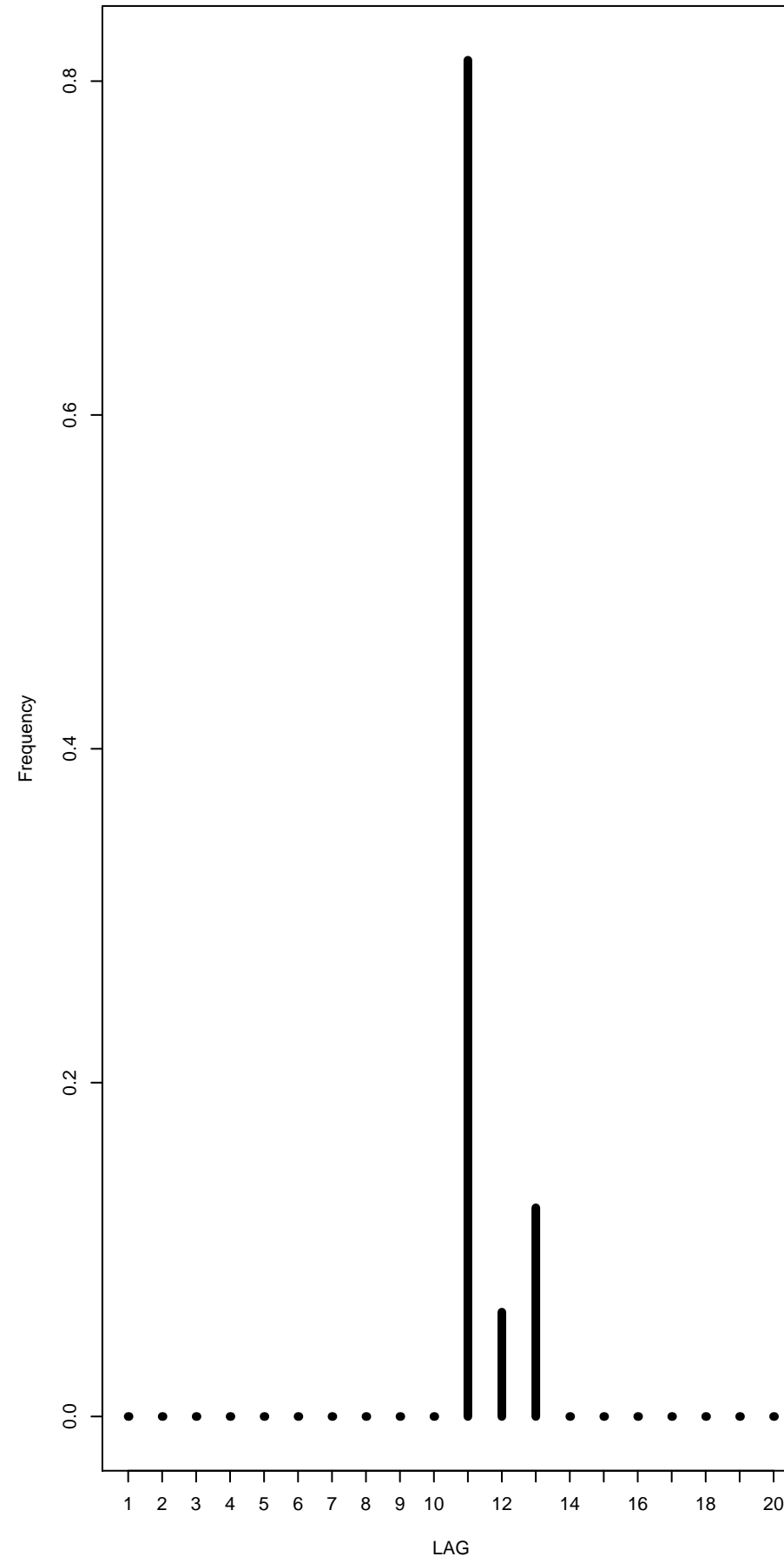
AIC n=1200
