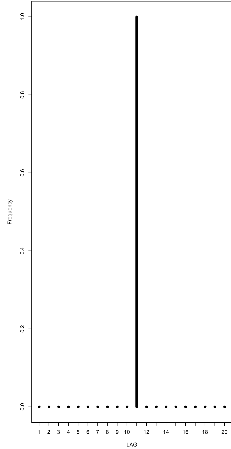
BIC n=600
