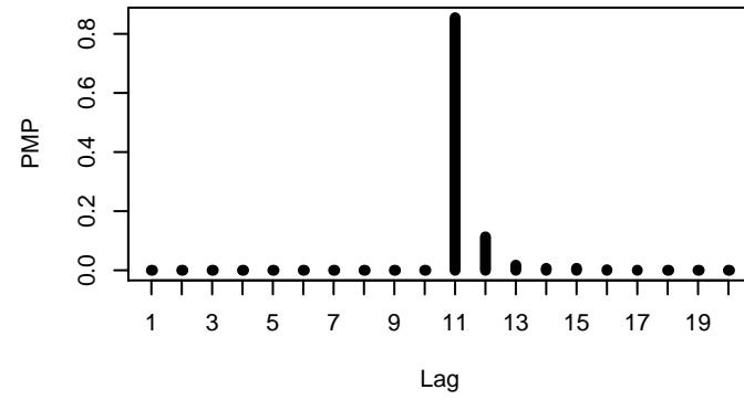
dataset 10 n=600
