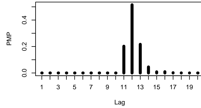
dataset 11 n=600
