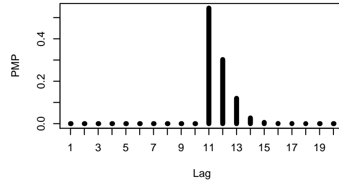
dataset 3 n=600
