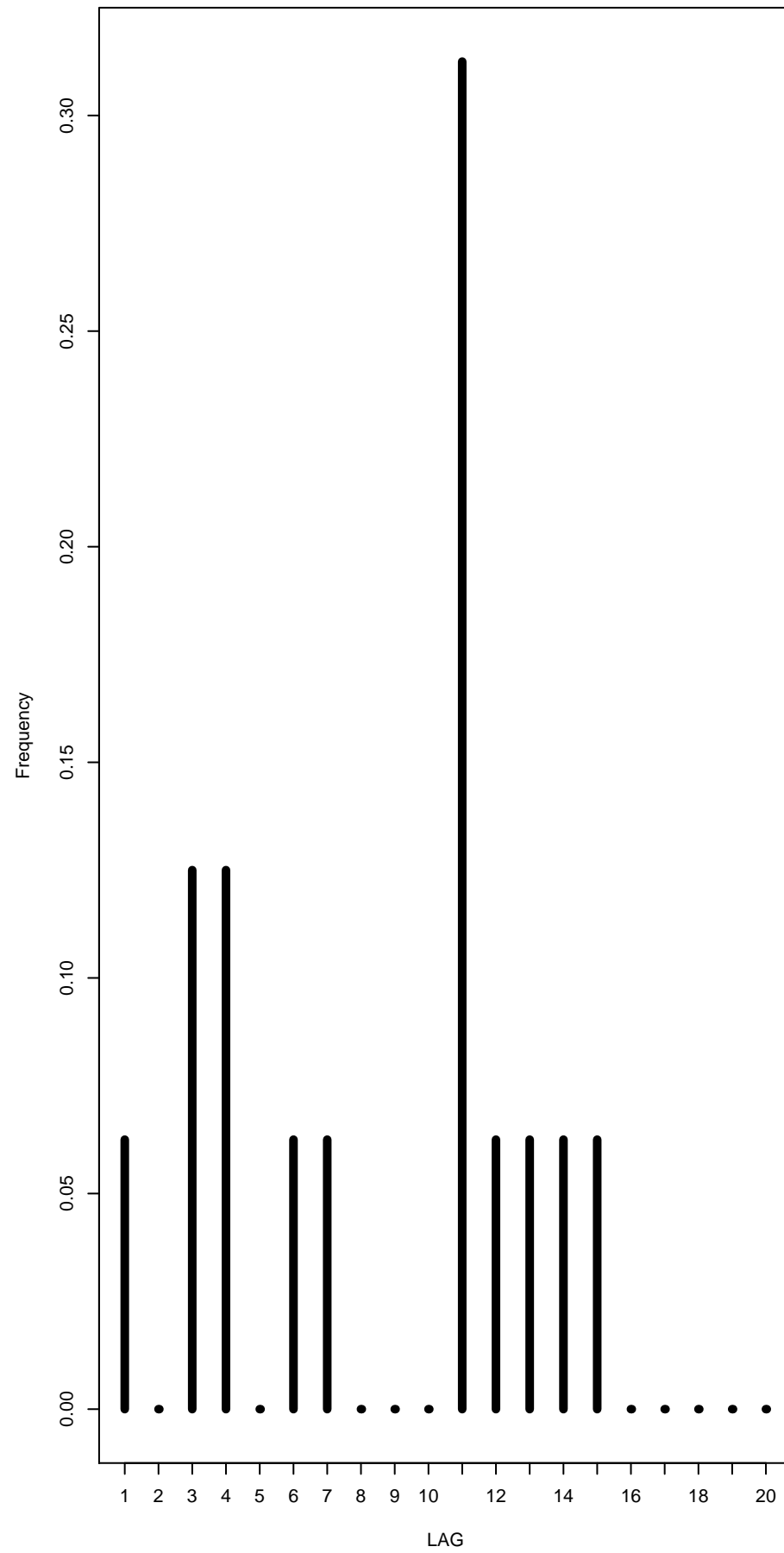
AIC n=120
