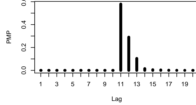
dataset 7 n=600
