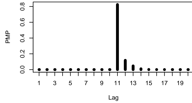
dataset 14 n=600
