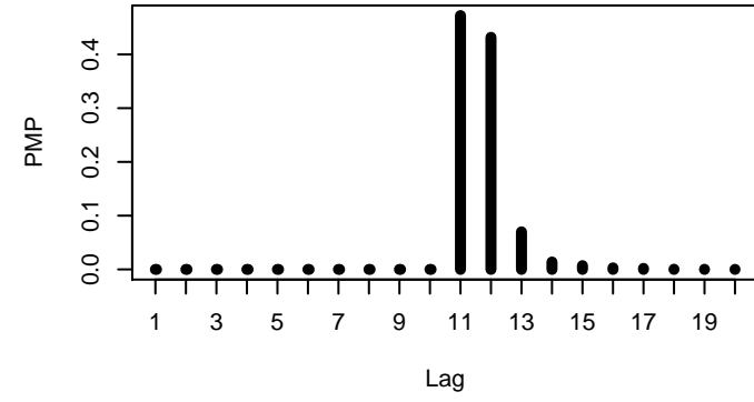
dataset 8 n=600
