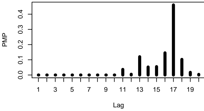
dataset 13 n=600
