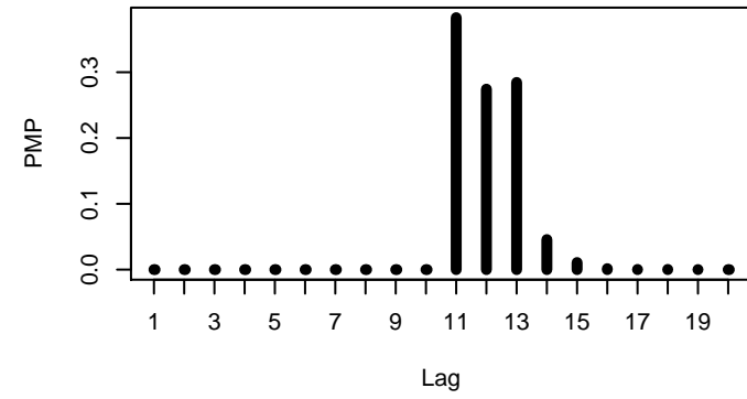
dataset 16 n=600
