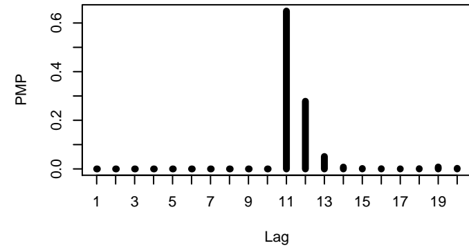
dataset 4 n=600
