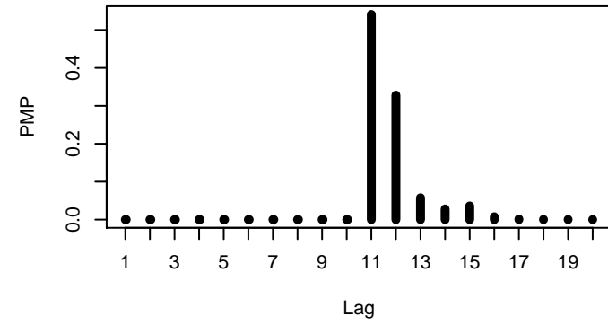
dataset 12 n=600
