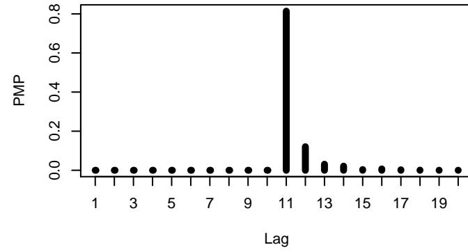
dataset 2 n=600
