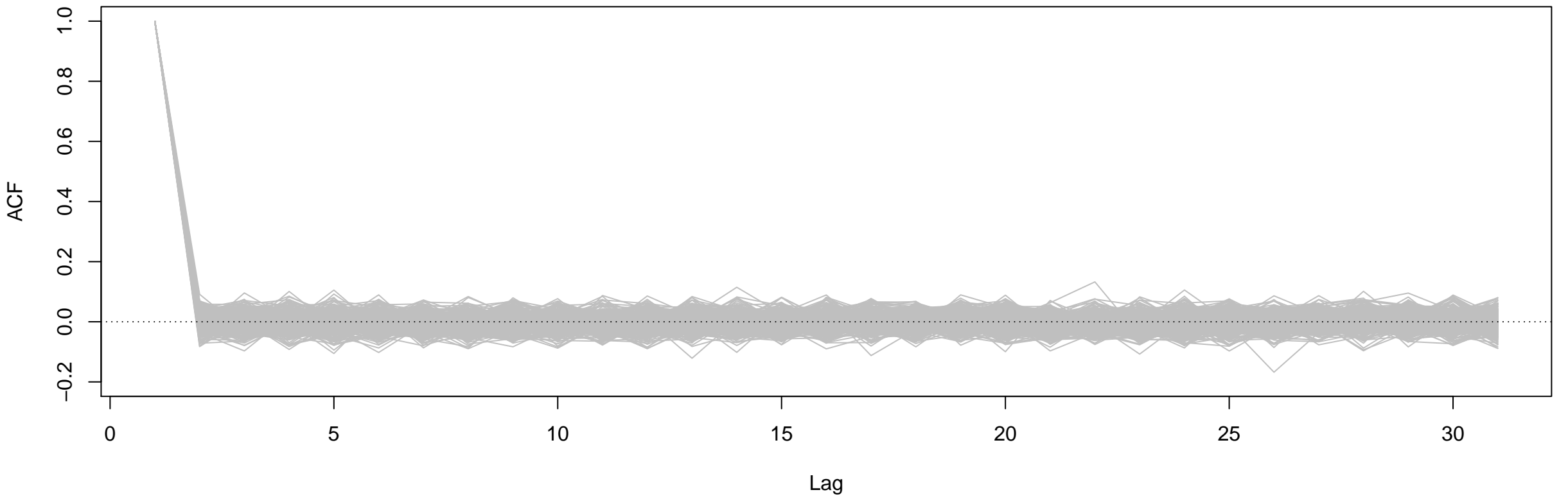
ACF for each x(t)
